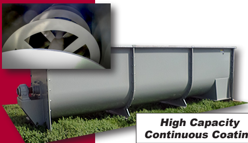
Continuous Mixer/Coater
